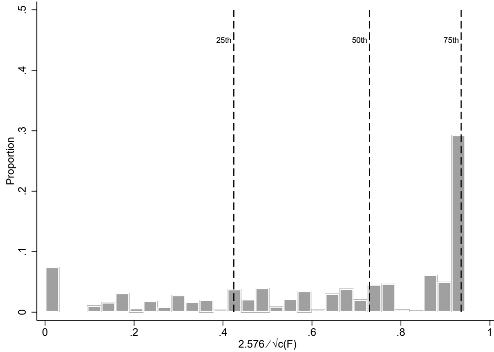
Figure 5b: Distribution of \frac{2.576}{\sqrt{c_{0.01}(F)}} for AER sample
