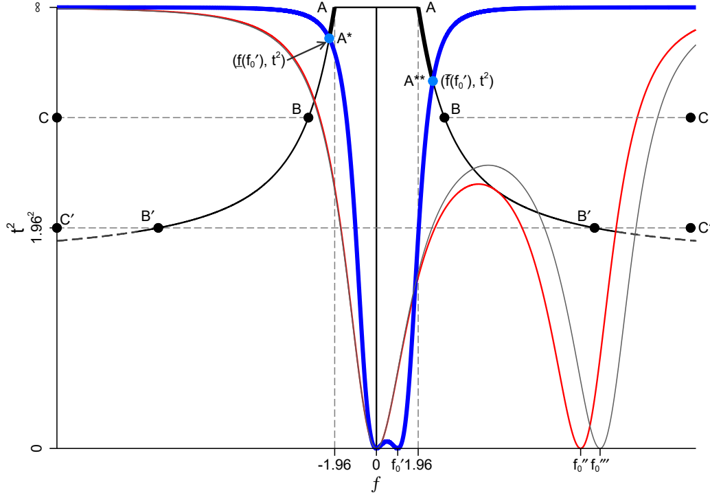
Figure 7: Construction of the tF Critical Value Function
