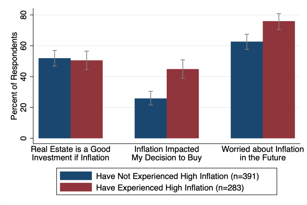
Figure IA.5. Inflation results by inflation experience.
