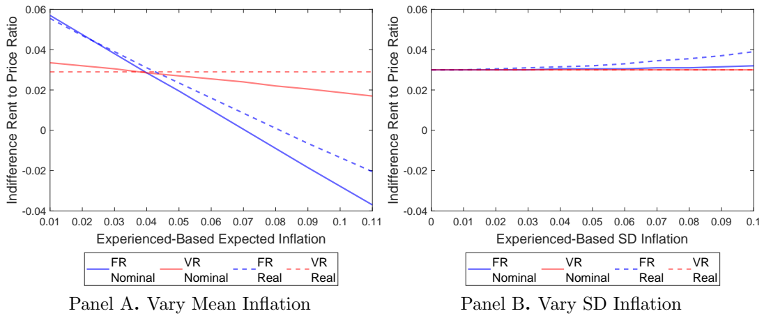
Figure IA.13. Simulations of experiences affecting the mean and variance of beliefs, normally distributed beliefs
