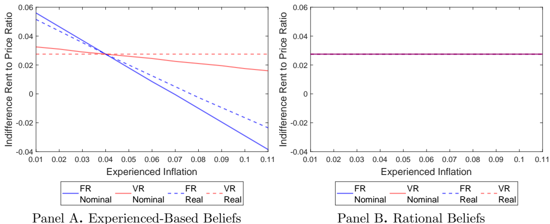
Figure IA.6. Simple simulation of the model
