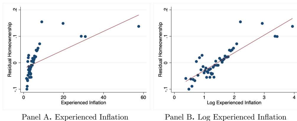
Figure 6. Binned Scatter Plots of Residual Homeownership and Inflation Experiences (HFCS)
