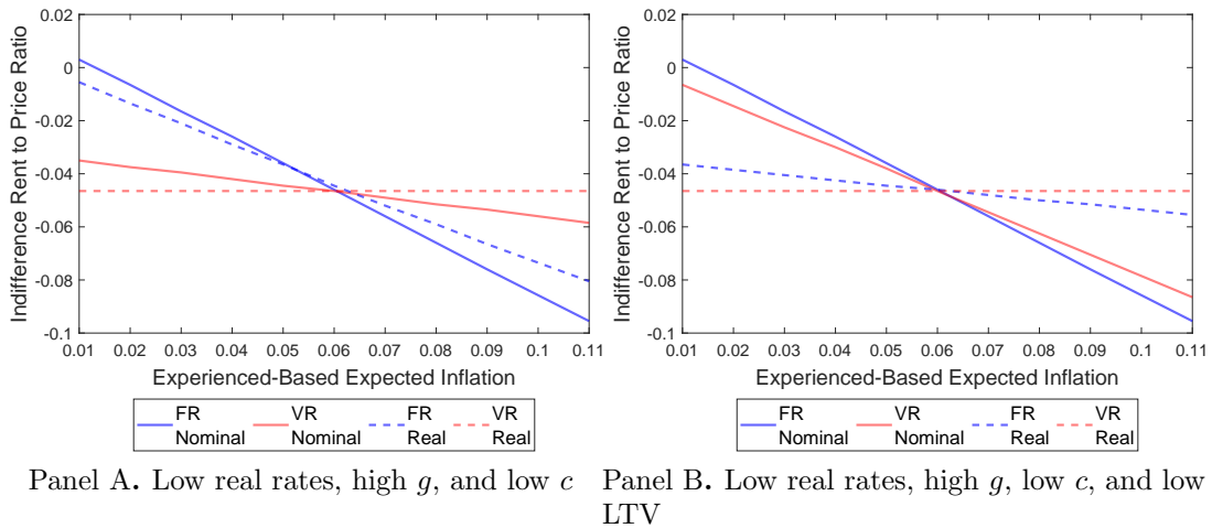
Figure IA.9. Stress tests of Prediction 2
