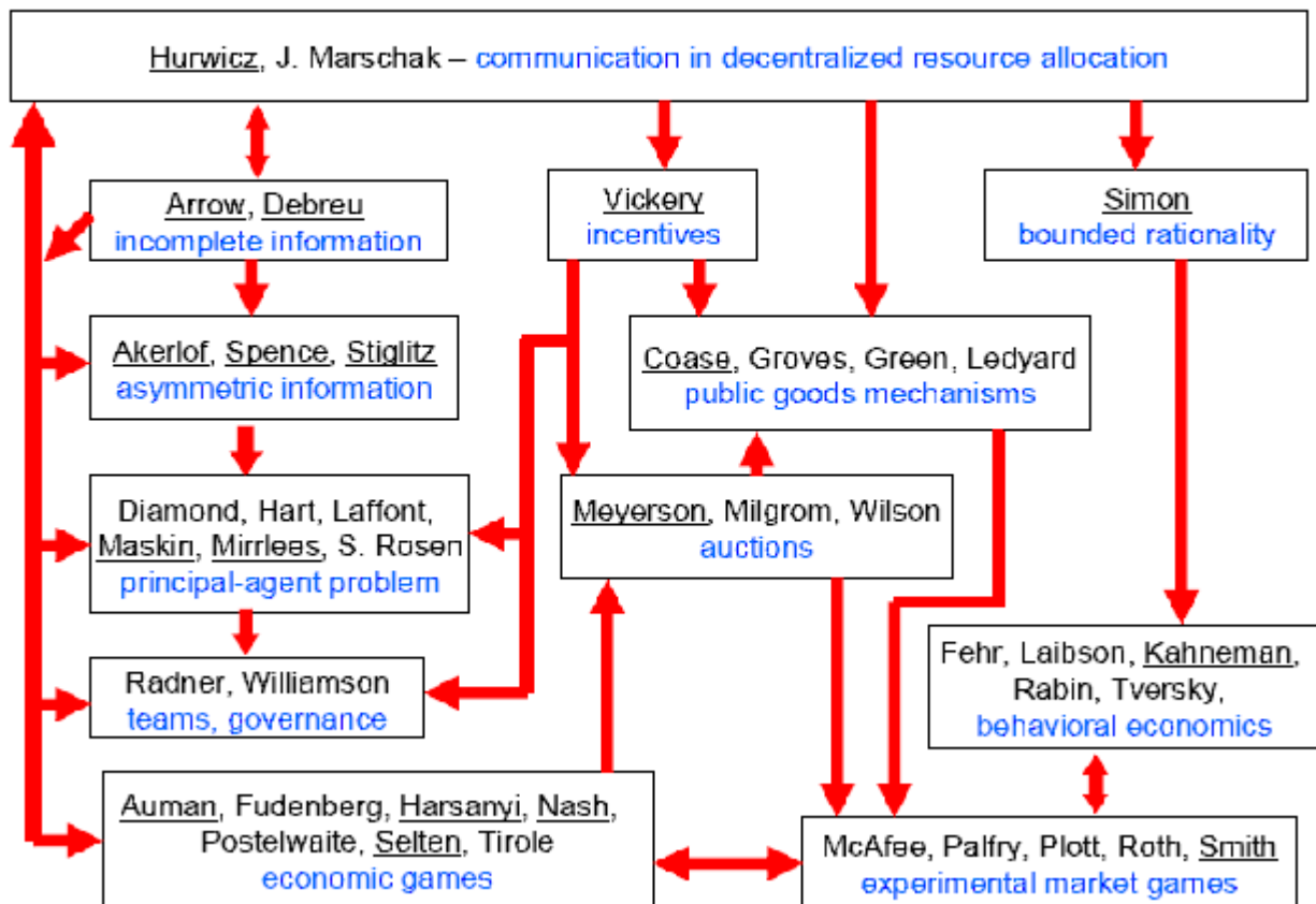
Figure 1. Mechanism Design in a Nutshell
