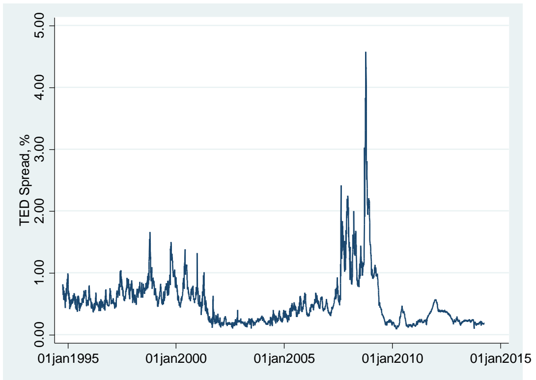
Figure 12. TED Spread.
