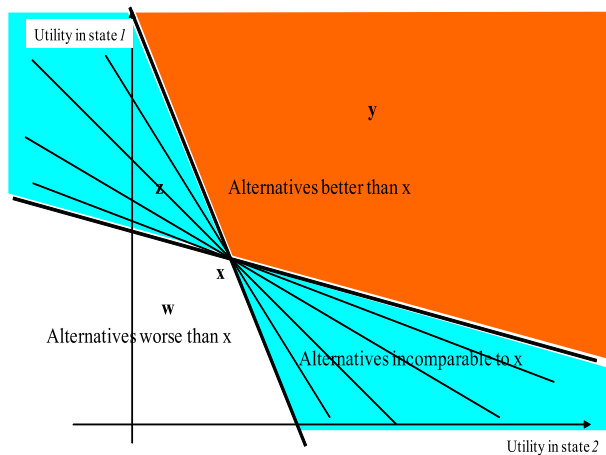
Fig. 1. Incomplete preferences.
