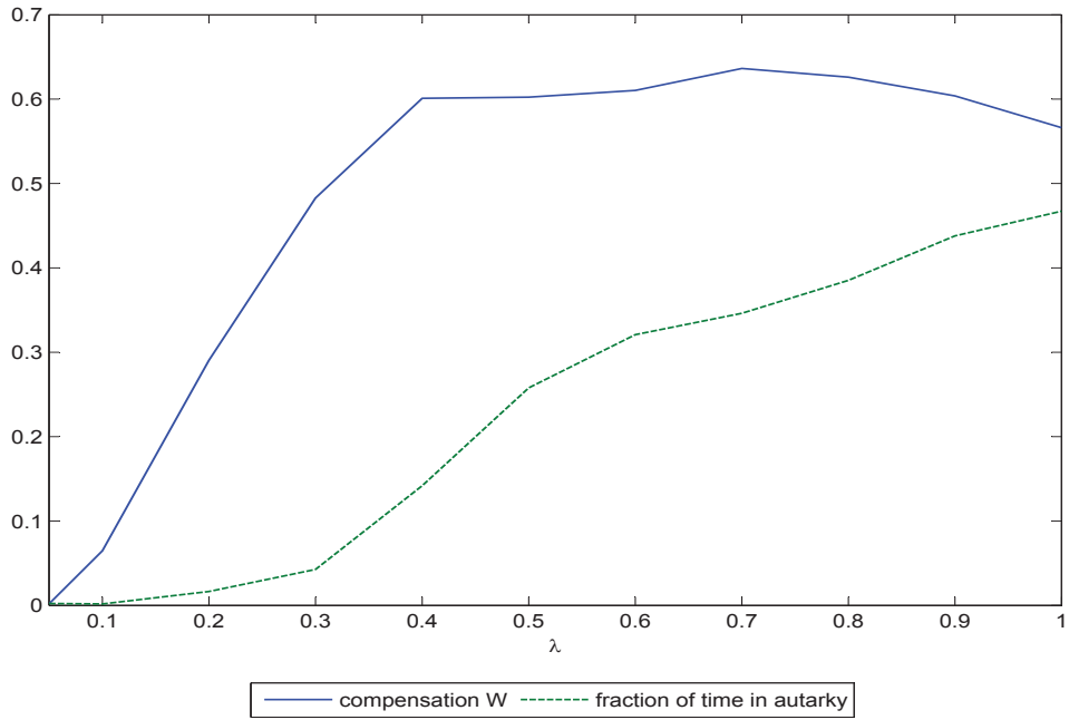
Figure 7.6: Consumption compensation W (solid blue) and fraction of time in autarky under ergodic distribution (dashed green) for different values of arrival probability of offers \lambda .
