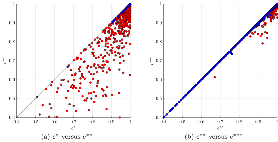
Figure 2: Scatterplots of Rationalizability Scores
