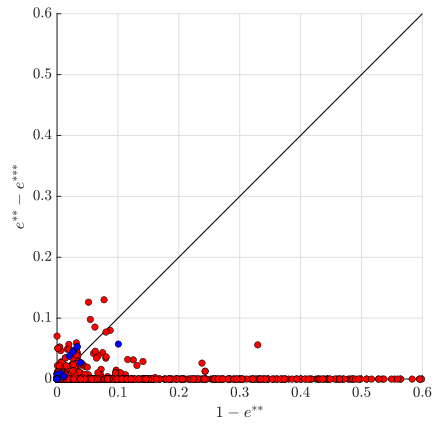
Figure 3: Scatterplots of Score Differences
