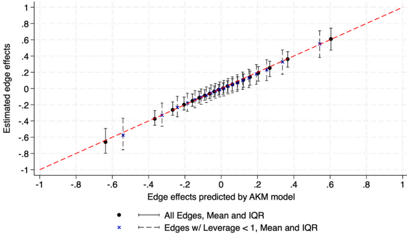
FIG. 2 Log daily wage change of edge ( \hat{\Delta} ) versus AKM prediction ( \tilde{\Delta} ). Notes: The vertical axis depicts binned averages of the elements of \hat{\Delta} : the average adjusted log daily wage changes associated with each origin-destination firm edge. The horizontal axis gives bins of \tilde{\Delta} : the wage change predicted by the least squares estimates of firm effects. Panel comprised of the 1999 and 2001 waves of the Veneto Work Histories dataset developed by the Economics Department in Università Ca' Foscari Venezia under the supervision of Giuseppe Tattara.
