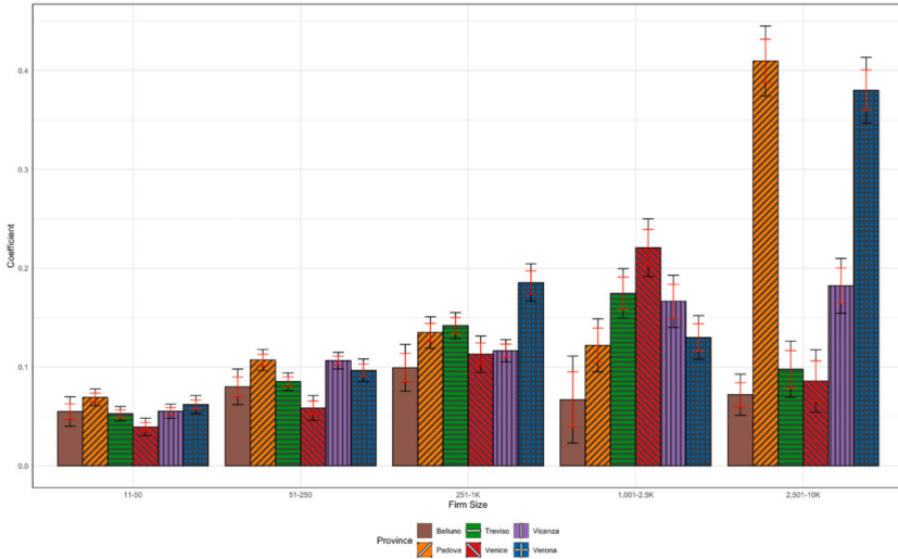
FIG. 4 Mean firm effects by firm size and province. Notes: Sample comprised of firms in leave-out connected set described in Table 2. Bar height gives coefficient from second step regression of firm effects onto province indicators plus interactions with indicators for firm size category. Omitted firm size category in each province is 1–10. Both confidence intervals derived by adding \pm 1.96 standard errors to the point estimate. Outer confidence interval (depicted in black) relies on (Z'Z)^{-1}Z'\hat{V}_\varepsilon[\hat{\psi}]Z(Z'Z)^{-1} as estimator of the asymptotic variance. Inner confidence interval (depicted in red) relies on \frac{J}{J-k}(Z'Z)^{-1}Z'\{\text{diag}(M_Z\hat{\psi})\}^2Z(Z'Z)^{-1} as estimator of the asymptotic variance, where M_Z = I - Z(Z'Z)^{-1}Z' .
