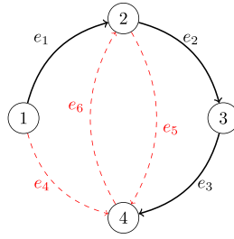
FIG. 1 A mobility network ( J = 4 , |E| = 6 ).
