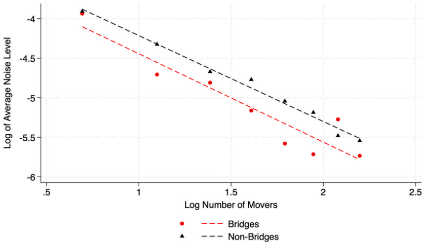
FIG. A.1 Noise level by number of movers per edge. Notes: The vertical axis depicts the natural logarithm of the average of \hat{V}[\hat{\Delta}_\varepsilon] among edges with a given number of movers. Number of movers considered ranges from 2 to 10. The line of best fit (depicted above) has intercept -3.325 and slope -1.118 when fit on edges that are bridges and an intercept of -3.126 and slope -1.087 when fit on edges that are not bridges. Using these lines of best fit to impute the variance of singleton edges, the imputed noise level of singleton bridges is \exp(-3.325) \approx 0.036 and the imputed noise level for singleton edges that are not bridges is \exp(-3.12) \approx 0.044 .
