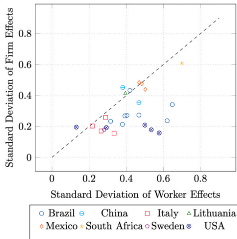
FIG. 3 Bias-corrected standard deviations of firm and worker fixed effects by country.
