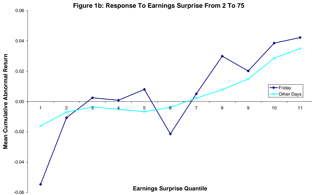
Figures 1a-1b. Stocks in CRSP are matched to quarterly earnings announcements in I/B/E/S from January 1995 until June 2006. In event time, day 0 is the day of the announcement. The cumulative abnormal return for each stock is the raw buy-and-hold return adjusted using the estimated beta from market model. The earnings surprise for an announcement is the difference between actual earnings for the quarter recorded by I/B/E/S and the median analyst forecast included in the I/B/E/S detail file during the 30 days before the quarterly earnings announcement scaled by the stock price 5 trading days before the announcement. Quantiles 1 through 5 contain earnings announcements for five quintiles of negative earnings surprises and quantiles 7 through 11 contain earnings surprises for five quintiles of positive earnings surprises. Quantile number 6 contains all announcements with an earnings surprise equal to zero. Since the number of negative earnings surprises, of positive earnings surprises, and of surprises equal to zero are unequal, the number of observations in each quantile differ. The breakpoints for the quantiles are determined separately for each year and announcements made on Saturday or Sunday are excluded from the sample.
