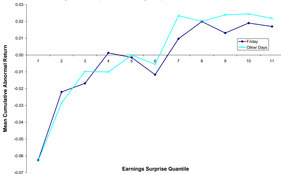
Figure 1d: Nonlinear Form of the Response to Earnings Surprise From 0 to 1
