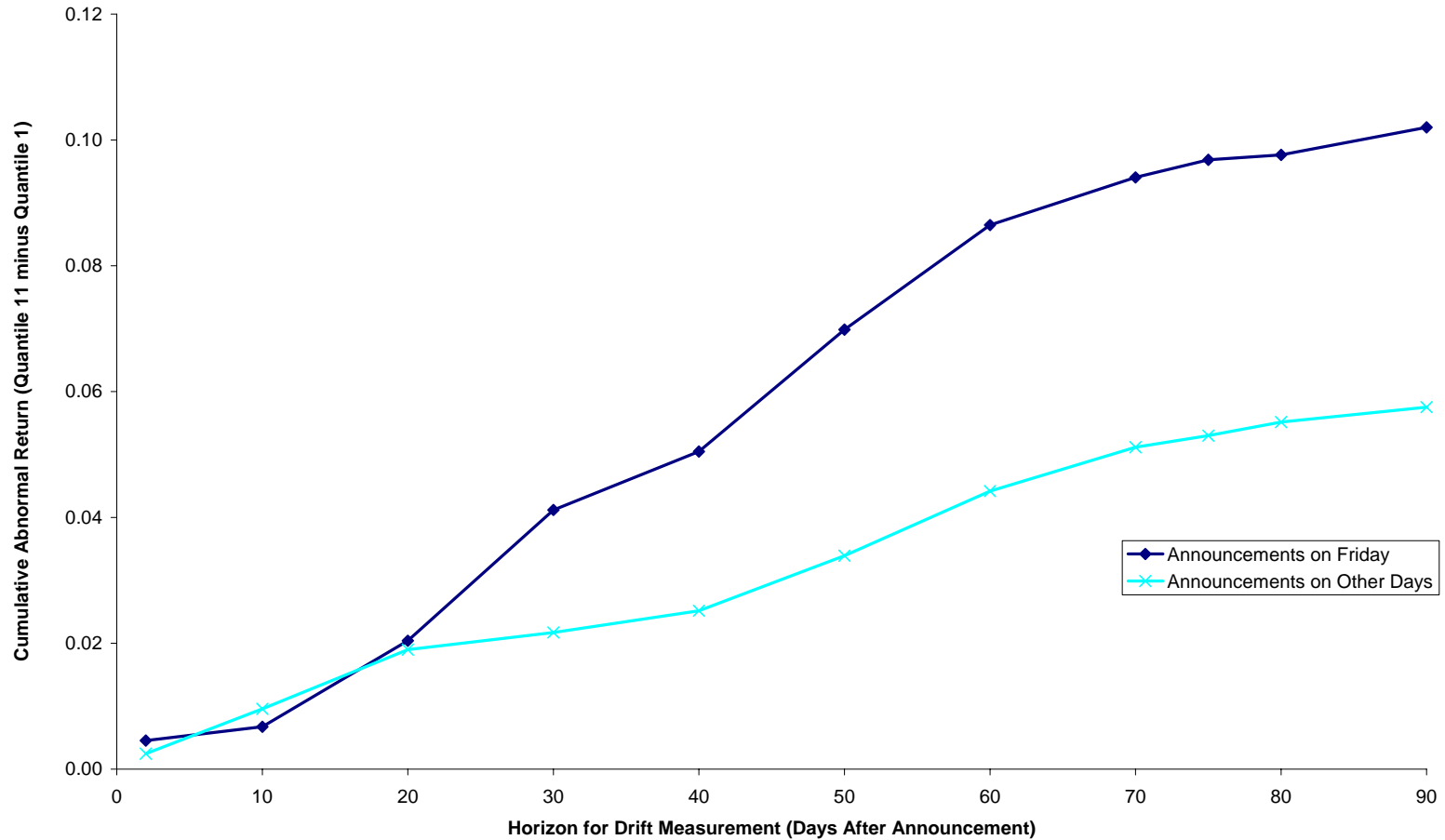
Figure 2. Stocks in CRSP are matched to quarterly earnings announcements in I/B/E/S from January 1995 until June 2006. In event time, day 0 is the day of the announcement. The cumulative abnormal return for each stock is the raw buy-and-hold return adjusted using the estimated beta from market model. The earnings surprise for an announcement is the difference between actual earnings for the quarter recorded by I/B/E/S and the median analyst forecast included in the I/B/E/S detail file during the 30 days before the quarterly earnings announcement scaled by the stock price 5 trading days before the announcement. Quantiles 1 through 5 contain earnings announcements for five quintiles of negative earnings surprises and quantiles 7 through 11 contain earnings surprises for five quintiles of positive earnings surprises. Quantile number 6 contains all announcements with an earnings surprise equal to zero. The breakpoints for the quantiles are determined separately for each year and announcements made on Saturday or Sunday are excluded from the sample. The measure for post-earnings announcement drift for horizon h is the average cumulative abnormal return from day 2 to day h for quantile 11 minus the average cumulative abnormal return from day 2 to day h quantile 1.
