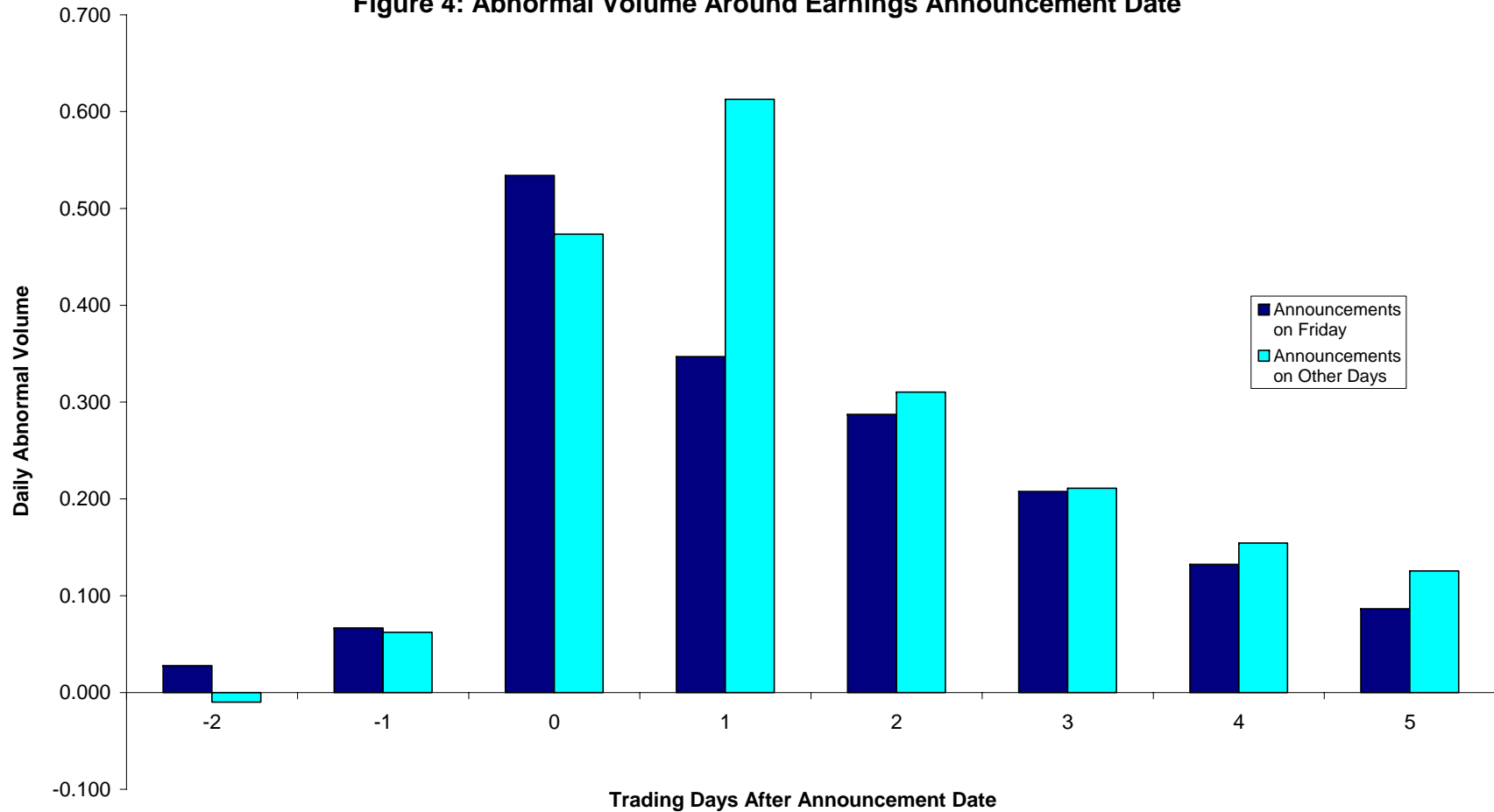
Figure 4. Stocks in CRSP are matched to quarterly earnings announcements in I/B/E/S from January 1995 until June 2006. In event time, day 0 is the day of the announcement. The abnormal volume for each stock is the average log volume on the day of and the day after the announcement, divided by the average log volume for the period -20 to -11 in event time (10 trading days). Announcements made on Saturday or Sunday are excluded from the sample.
